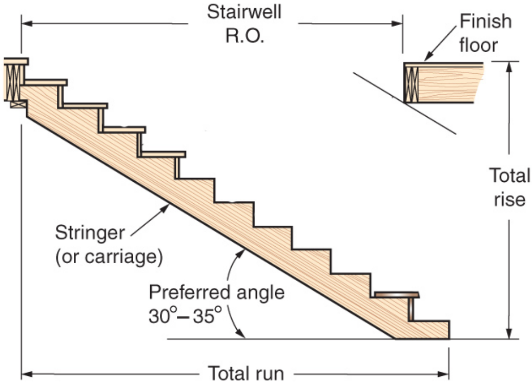
Figure 18-5. Basic stair parts and terms. The total number of risers is always one greater than the total number of treads.
